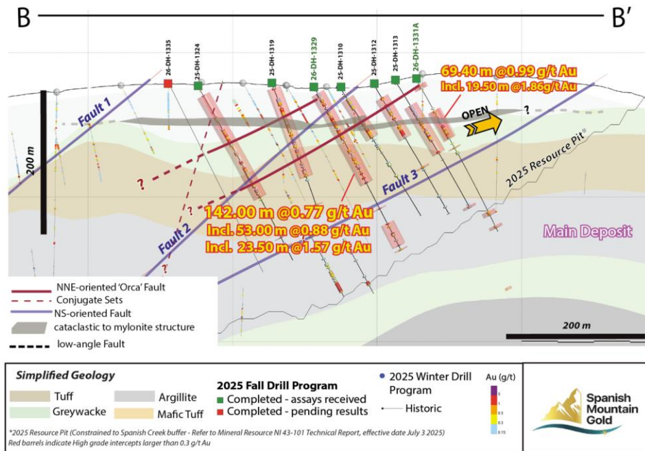
Figure 2: Drill Cross Section Through Orca Fault Area (looking northwest); section line B-B' (see Figure 3)
