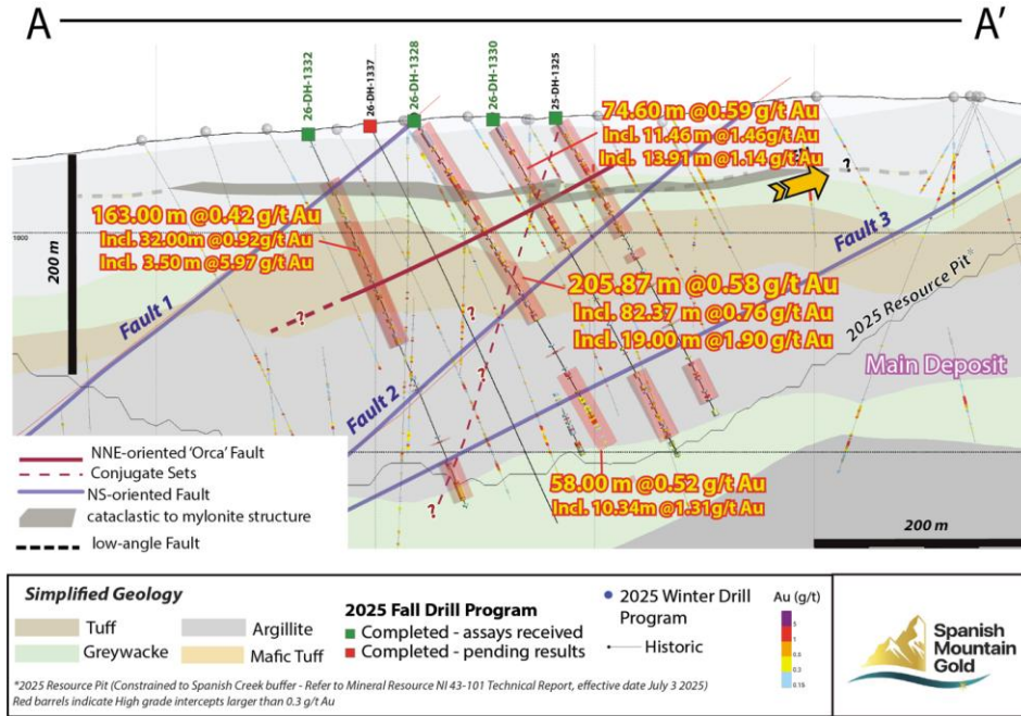
Figure 1: Drill Cross Section Through Orca Fault Area (looking northeast); section line A-A' (see Figure 3)
