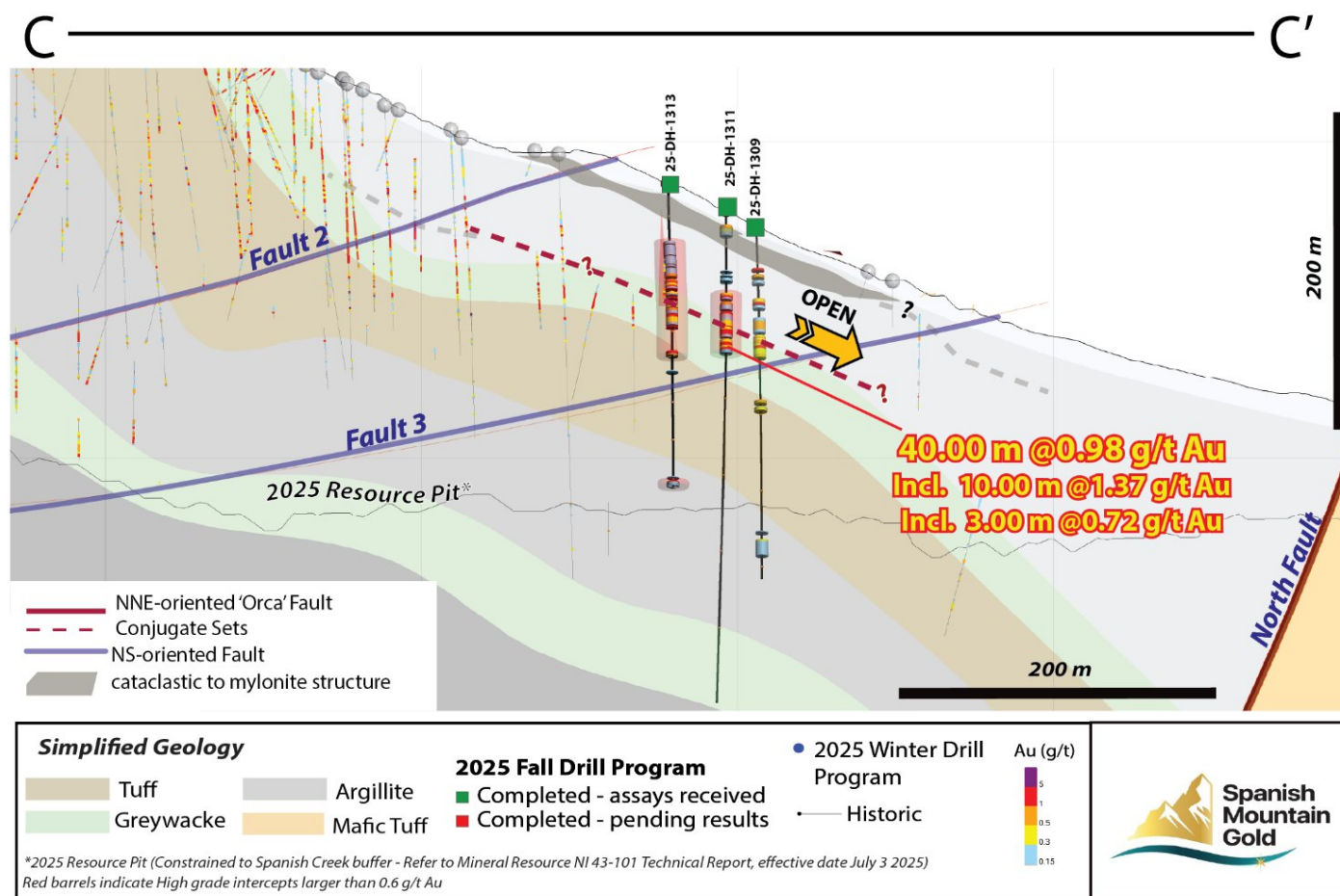
Figure 3: Drill Cross Section Through Orca Fault Area (looking northwest); section line C-C' (see Figure 4)
