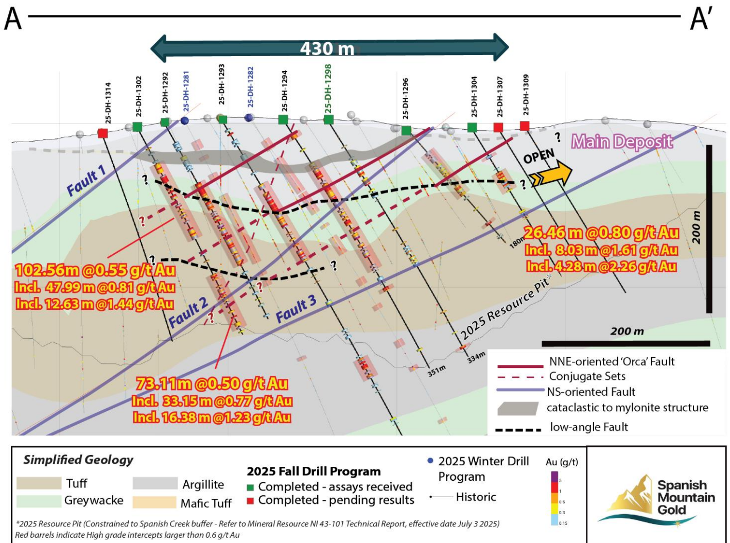
Figure 1: Drill Long Section Through Orca Fault Area (looking northeast); section line A-A' (see Figure 3)
