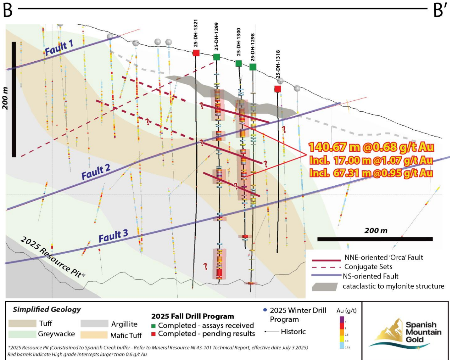
Figure 2: Drill Cross Section Through Orca Fault Area (looking northwest); section line B-B' (see Figure 3)
